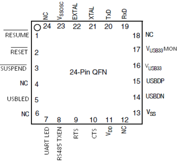
Figure 2. USB2SER — 24-QFN Package
