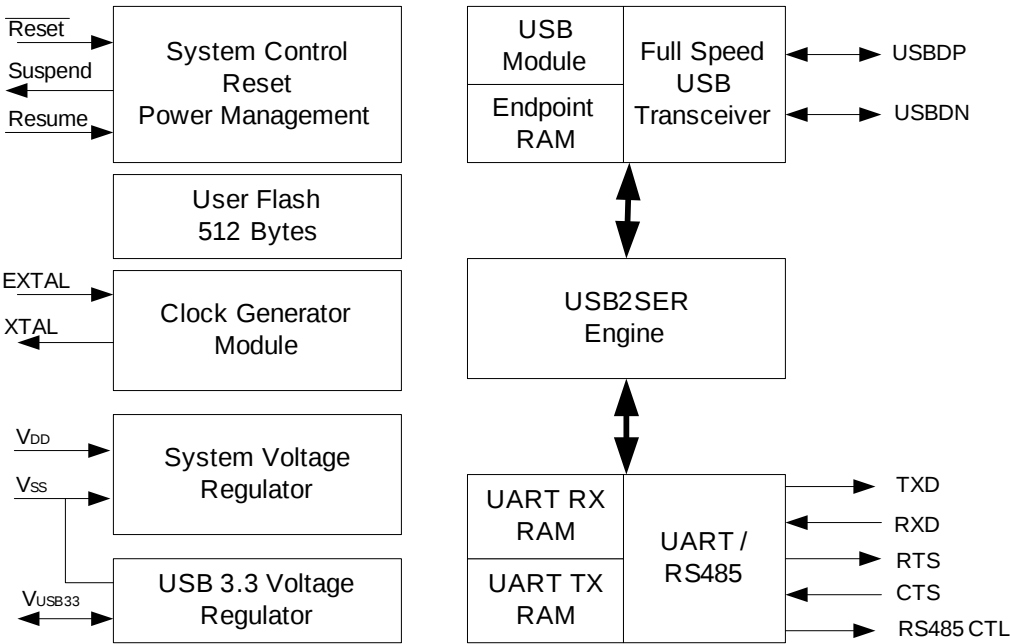
Figure 1. Device block diagram
