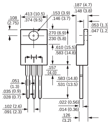
TO-220
