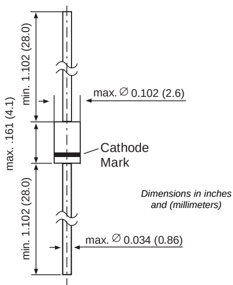
DO-204AL (DO-41 Glass)
