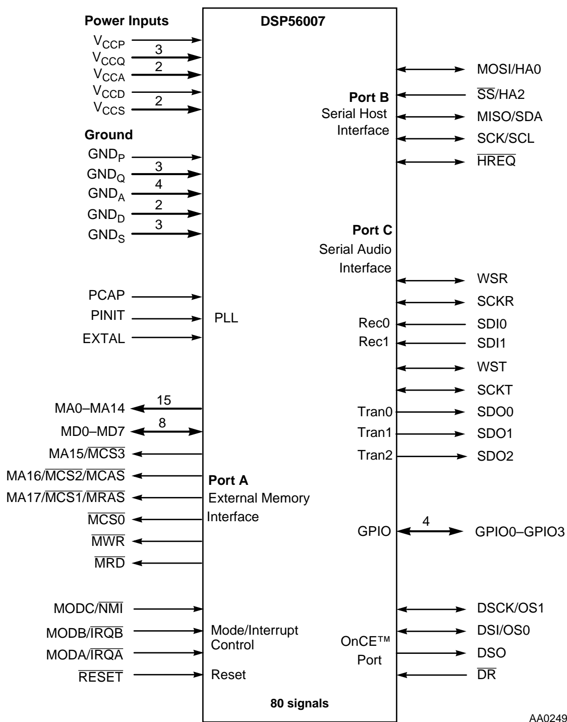
Figure 1-1 DSP56004 Signals
