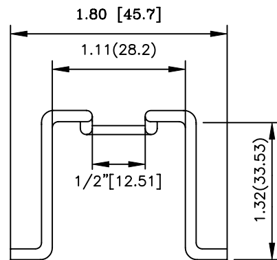
CLIP .072" Dia. Stainless Steel Wire
