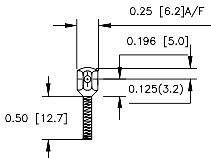
SCREW 6 BA Brass, Nickel Plated
