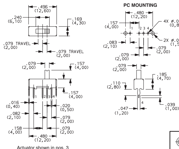
OS103011MS8QP1 SP3T
