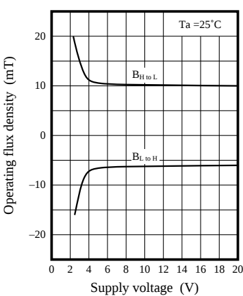
Operating flux density – Supply voltage
