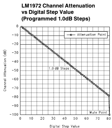
FIGURE 4. LM1972 1.0dB Attenuation Step Scheme
