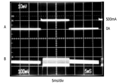
LOAD-TRANSIENT RESPONSE
