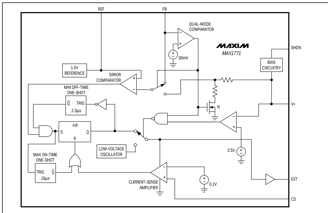
Figure 1. Functional Diagram
