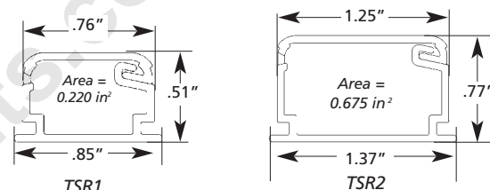
TSR Product Dimensions
