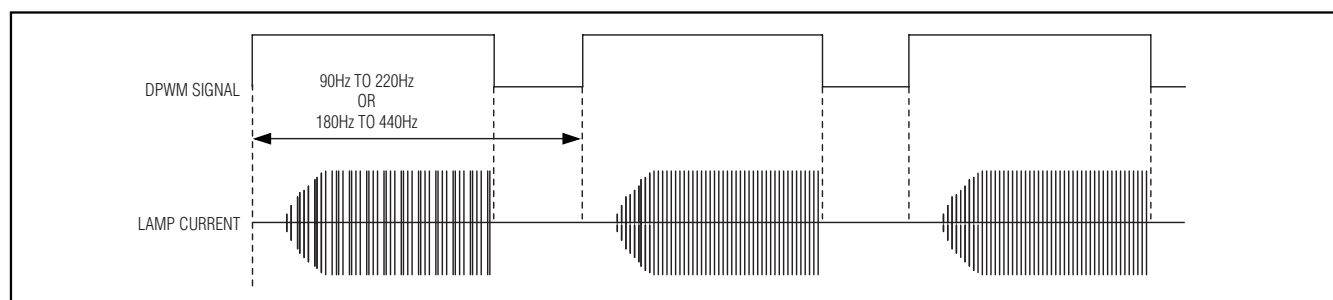
Figure 3. Digital-PWM Dimming and Soft-Start
