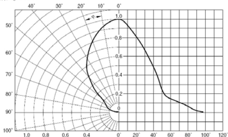
Radiation Characteristic
