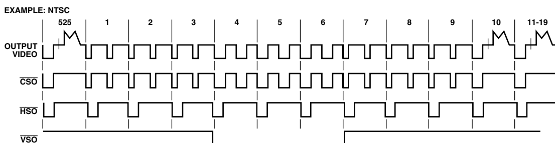
Figure 37. \overline{\text{CSO}} , \overline{\text{HSO}} , \overline{\text{VSO}} Timing Diagram
