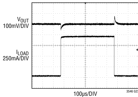
OUT1 Load Step
