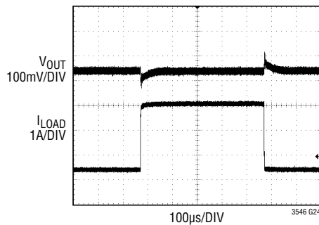
OUT2 Load Step
