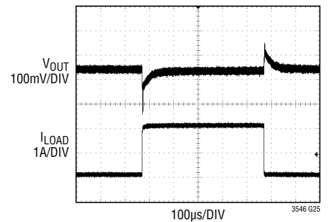
OUT2 Load Step
