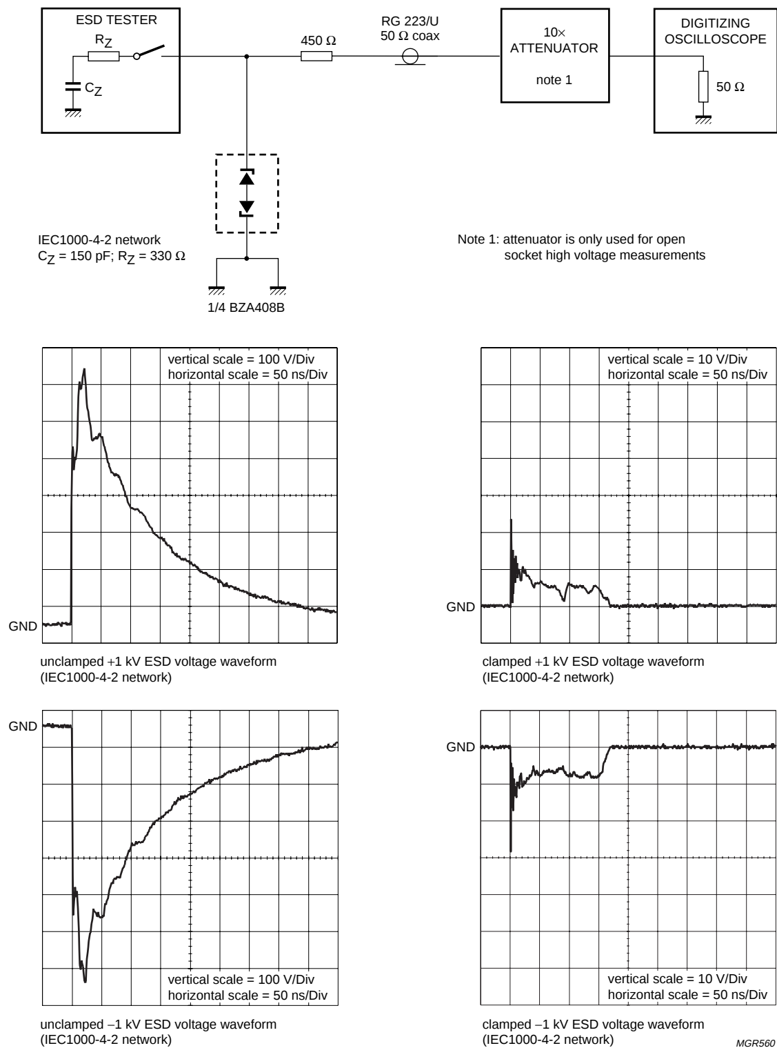
Fig.5 ESD clamping test set-up and waveforms.
