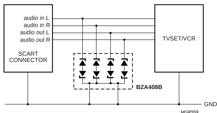
Fig.6 Scart connector protection.
