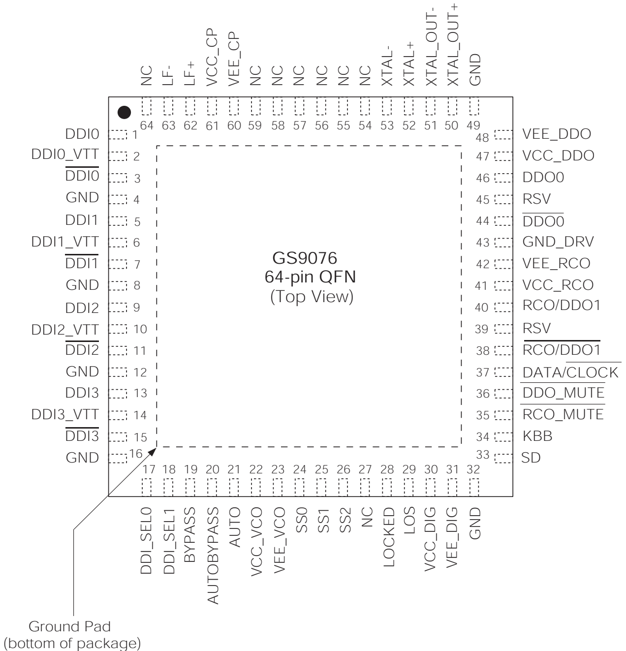
Figure 1-1: 64-Pin QFN
