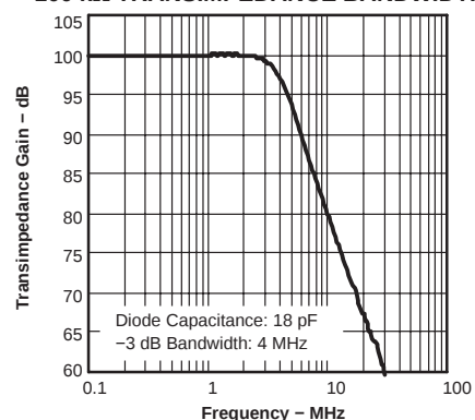
100 k \Omega TRANSIMPEDANCE BANDWIDTH
