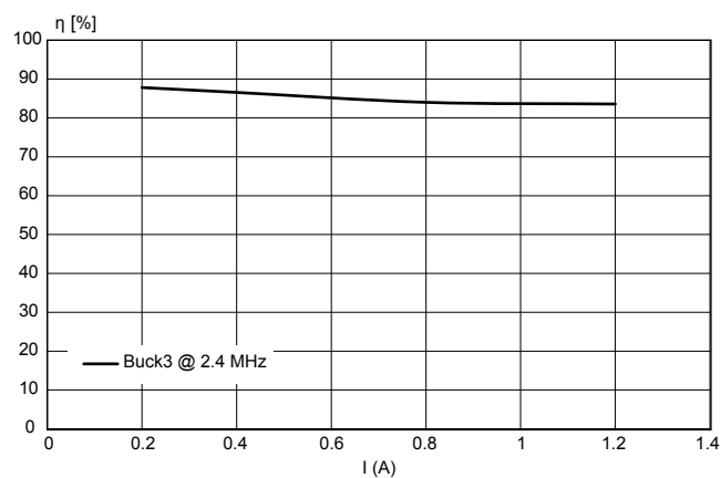
Figure 5. Efficiency of Buck3 with V_{in} = 3.3\text{ V} and V_{out} = 2\text{ V}
