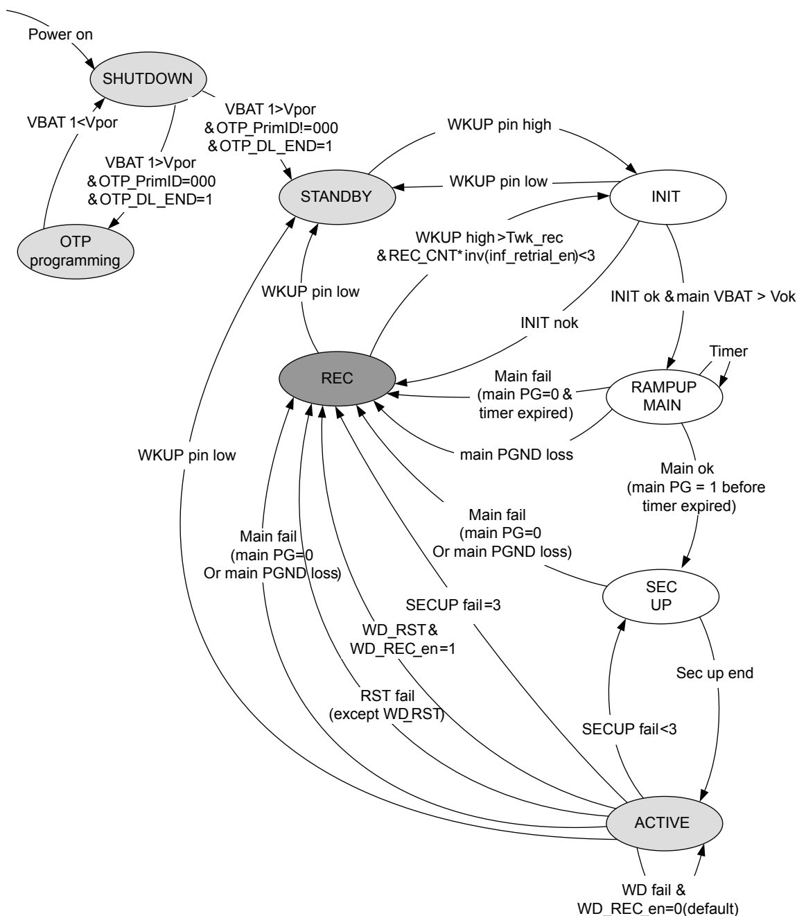
Figure 24. State machine
