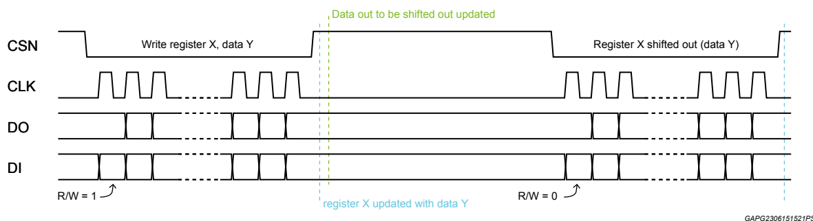
Figure 22. SPI protocol diagram
