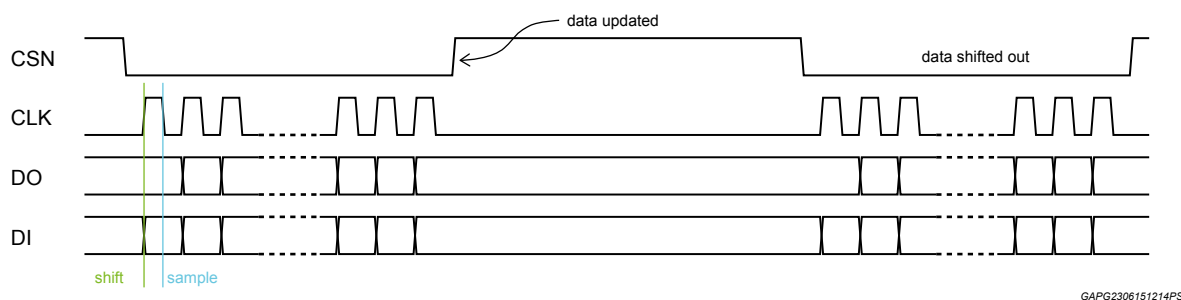
Figure 21. SPI diagram
