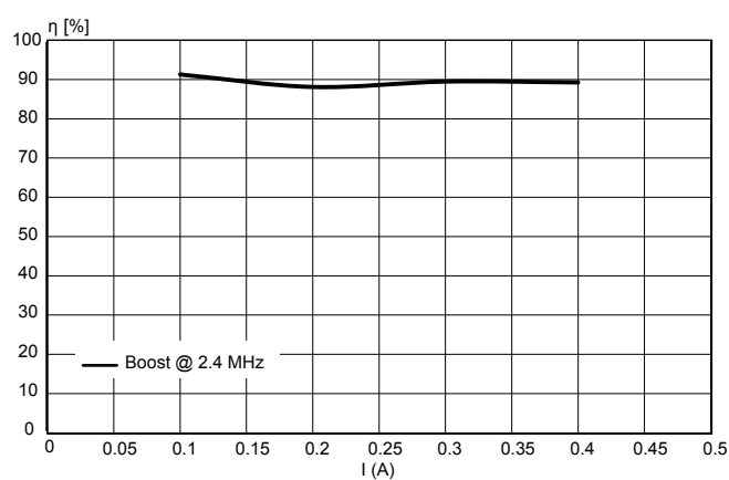
Figure 7. Efficiency of Boost with V_{in} = 3.3\text{ V} and V_{out} = 5\text{ V}
