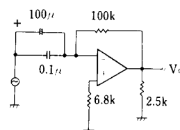
Test Circuit
