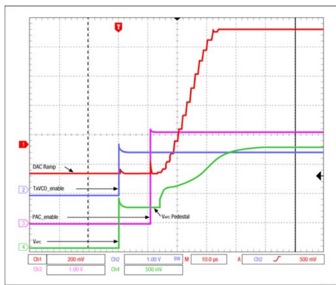
Figure 13. GSM Transmitter – Typical Ramp-up Signals
