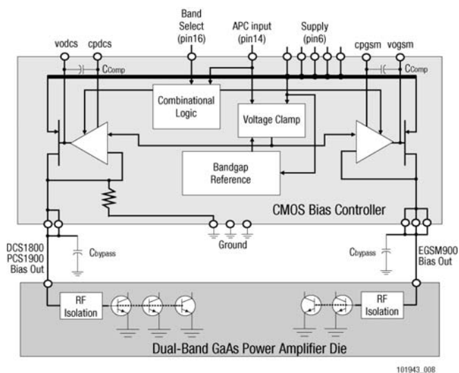
Figure 8. Functional Block Diagram
