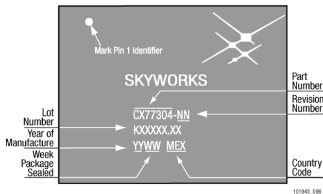
Figure 6. Typical Case Markings
