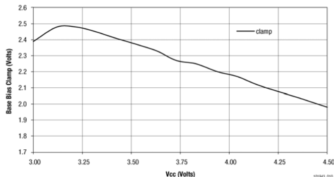
Figure 10. Base Bias Clamp Voltage vs. Supply Voltage
