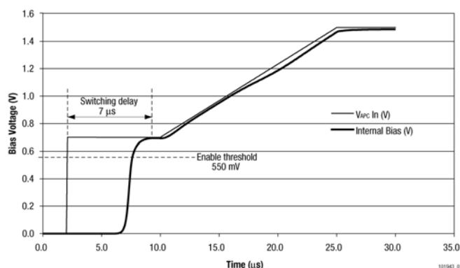
Figure 12. PAM Internal Bias Performance—Pedestal Applied
