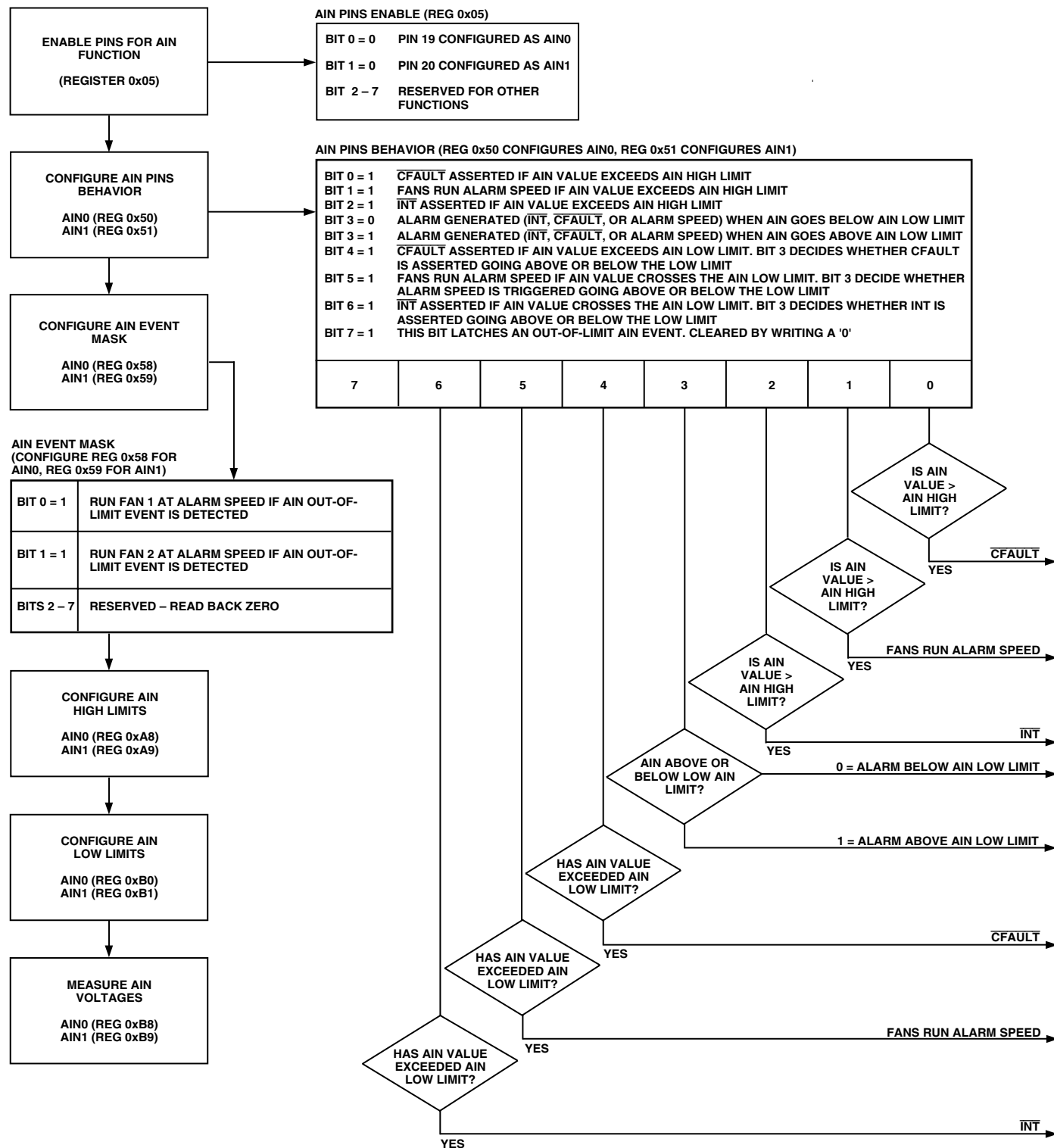
Figure 18. Configuring AIN0 and AIN1 Pins
