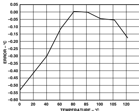
TPC 13. Local Temperature Error
