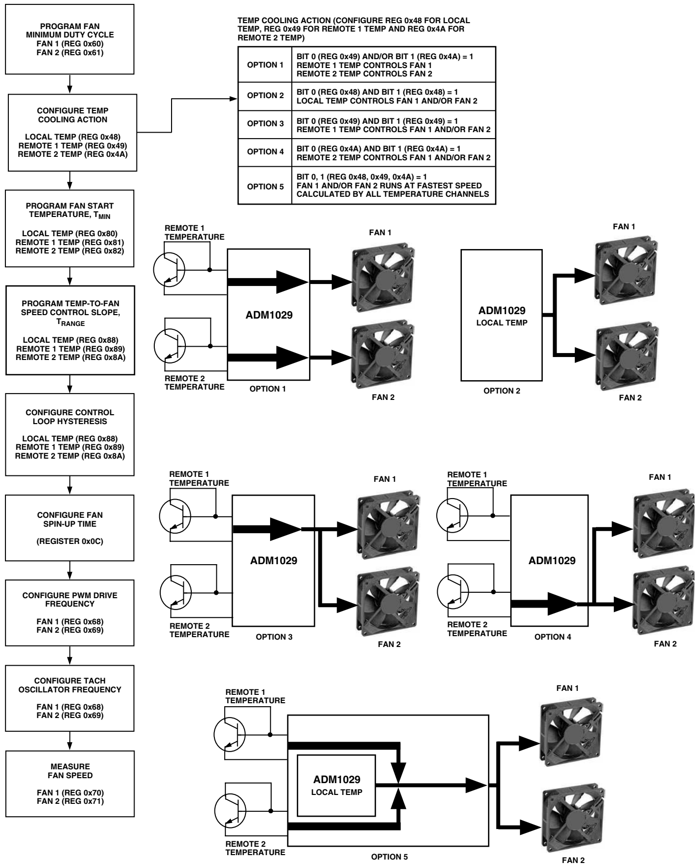
Figure 15. Configuring Automatic Fan Speed Control
