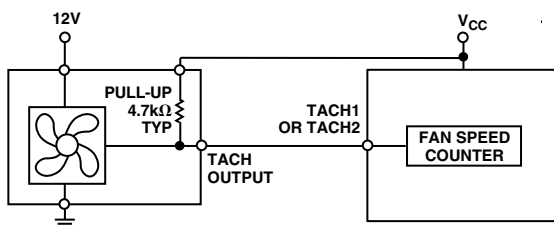
Figure 9a. Fan with Tach Pull-Up to +V_{CC}
