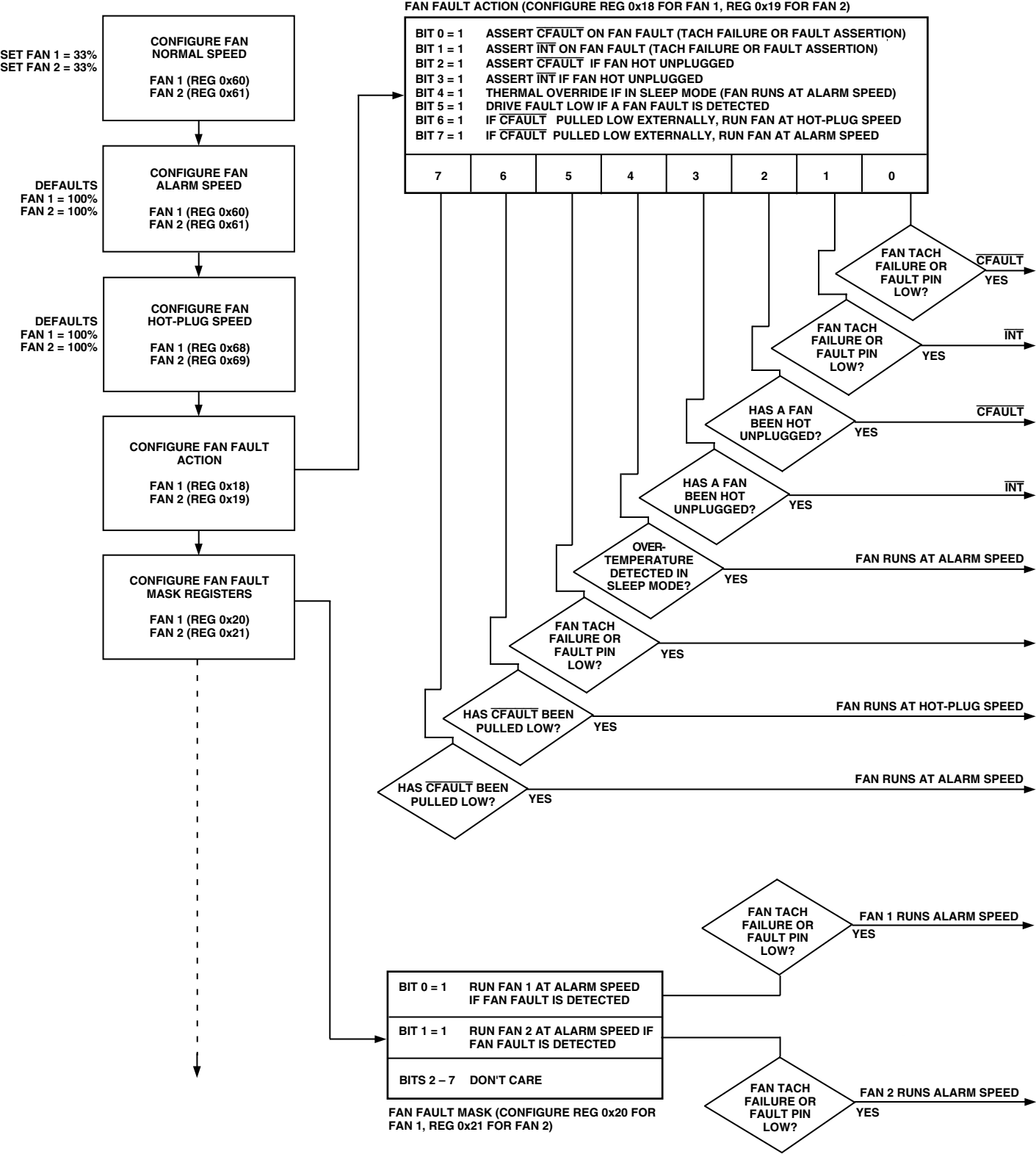
Figure 16. Fan Configuration Flowchart
