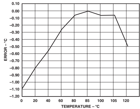
TPC 12. Remote Temperature Error
