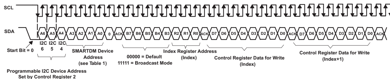
Figure 27. I 2 C Write Sequence
