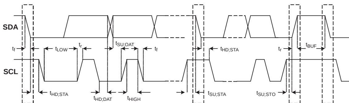
Figure 3. I²C / S²C Timing
