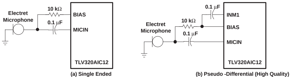
Figure 21. Microphone Interface
