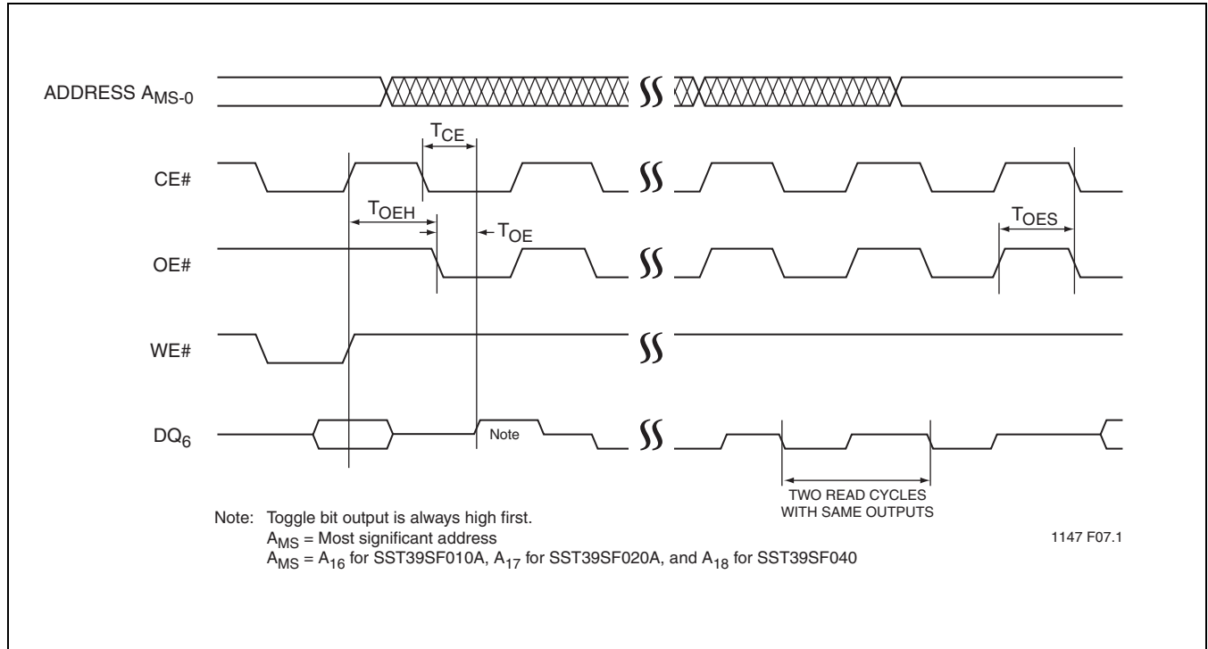
FIGURE 9: Toggle Bit Timing Diagram
