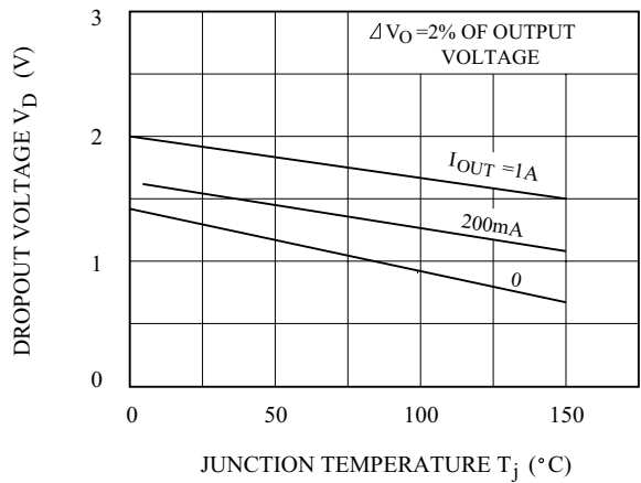
V_D - T_j
