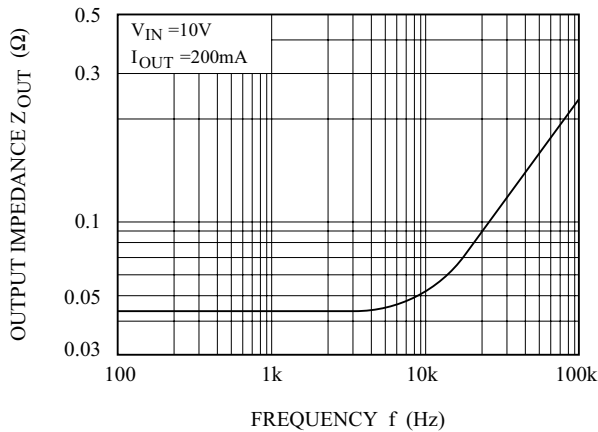
Z_{OUT} - f
