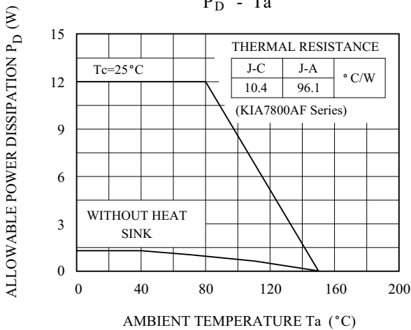
P_D - T_a
