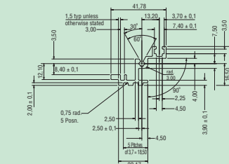
Handle Extrusion
