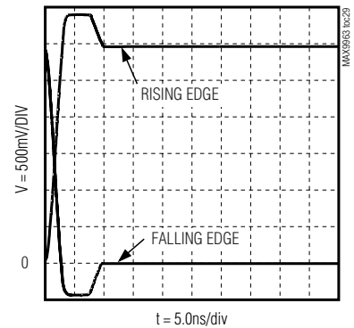
CLAMP RESPONSE
