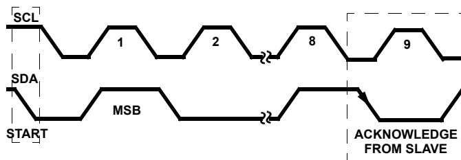
FIGURE 4. ACKNOWLEDGE ON THE I 2 C BUS
