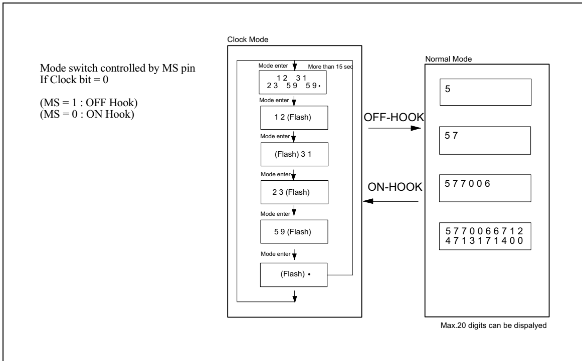
Figure 5. Mode Chart
