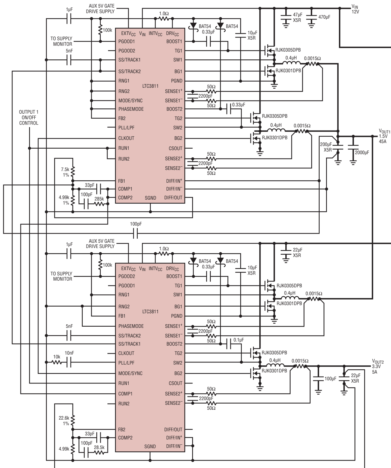
Figure 31. 3-Phase, 12V Input, 1.5V/45A Output with a 3.3V/5A Auxiliary Output
