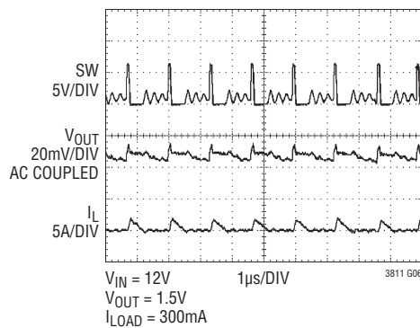
Light Load Waveforms (Pulse Skip Mode)
