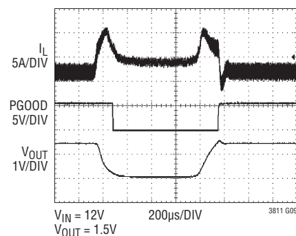
Short-Circuit Waveforms
