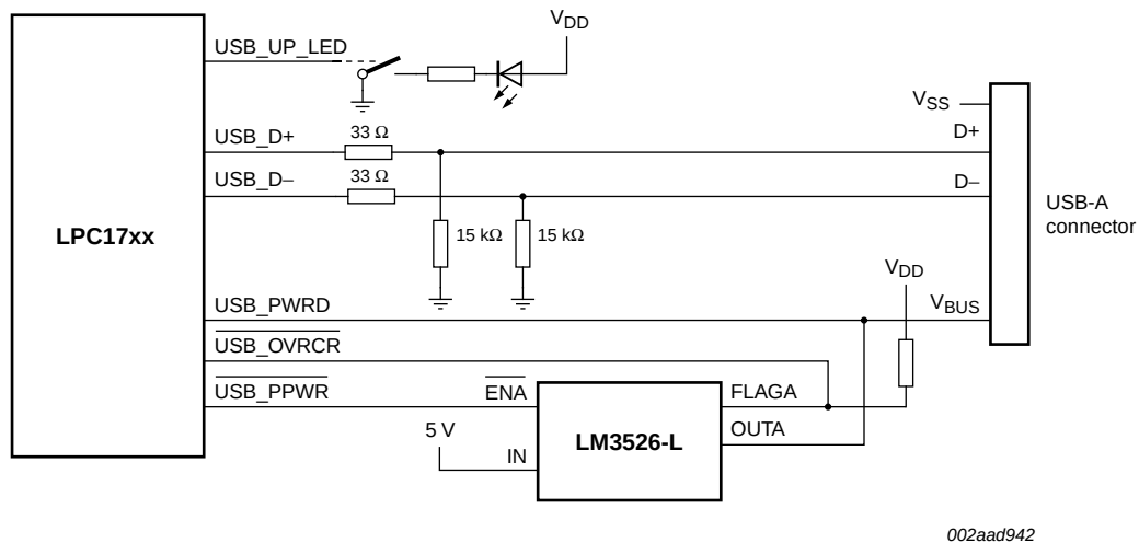
Fig 34. USB host port configuration
