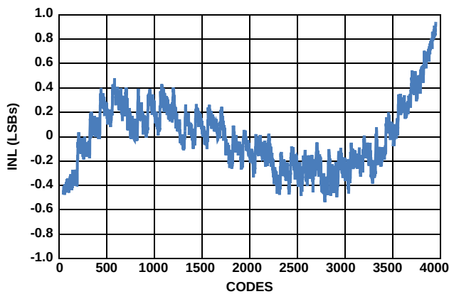
FIGURE 11. INTEGRAL NONLINEARITY
