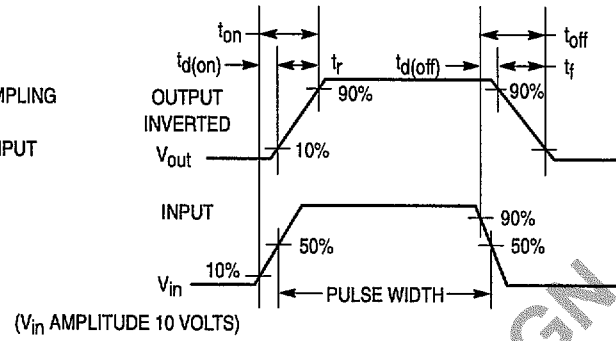
Figure 2. Switching Waveform
