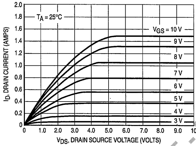
Figure 3. Ohmic Region
