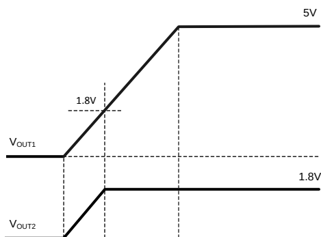
Figure 22. Tracking with Equal Slew Rates
