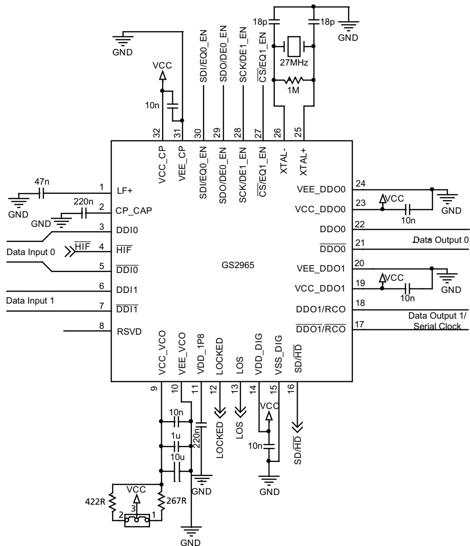
Figure 5-1: GS2965 Typical Application Circuit
