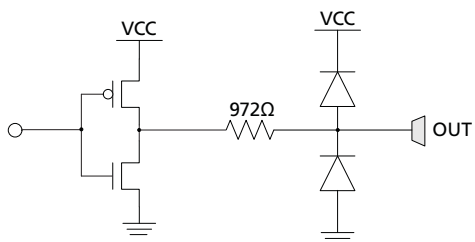
Figure 3-3: Low-speed Outputs (LOCKED, LOS, SD/ \overline{\text{HD}} )
