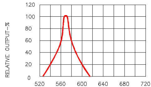
Fig.2 SPECTRAL RESPONSE
