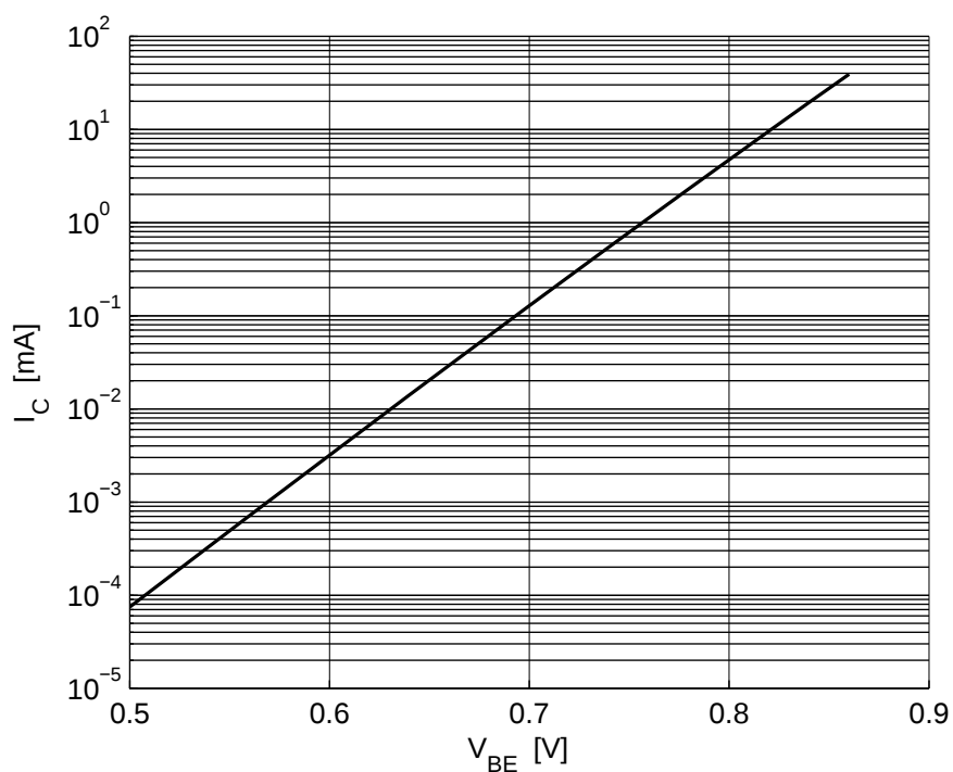
Figure 5-4 Collector Current vs. Base Emitter Forward Voltage I_C = f(V_{BE}) , V_{CE} = 2.5 V
