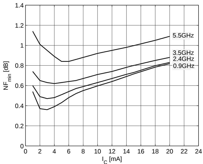
Figure 5-20 Noise Figure NF_{min} = f(I_C) , V_{CE} = 2.5\text{ V} , Z_S = Z_{opt} , f = \text{Parameter in GHz}
