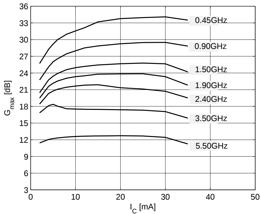
Figure 5-13 Maximum Power Gain G_{\max} = f(I_C) , V_{CE} = 2.5\text{ V} , f = \text{Parameter in GHz}
