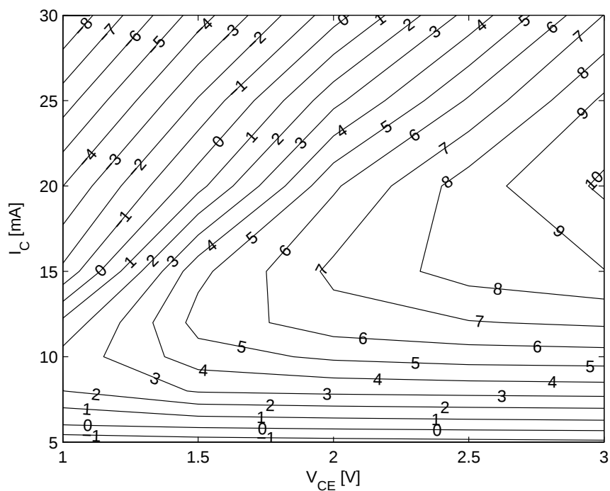
Figure 5-10 Compression Point at output OP_{1dB} [dBm] = f(I_C, V_{CE}) , Z_S = Z_L = 50 \Omega , f = 3.5 \text{ GHz}
