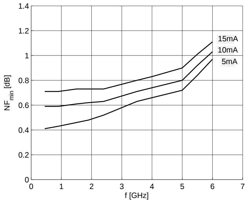
Figure 5-19 Noise Figure NF_{min} = f(f) , V_{CE} = 2.5\text{ V} , I_C = 5 / 10 / 15\text{ mA} , Z_S = Z_{opt}
