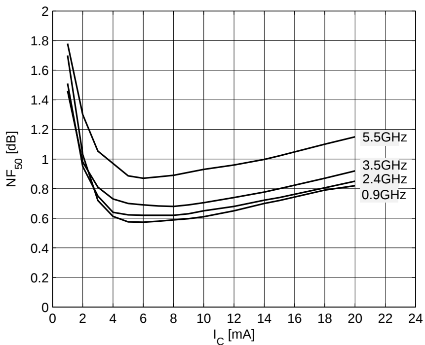
Figure 5-21 Noise Figure NF_{50} = f(I_C) , V_{CE} = 2.5\text{ V} , Z_S = 50\ \Omega , f = \text{Parameter in GHz}
