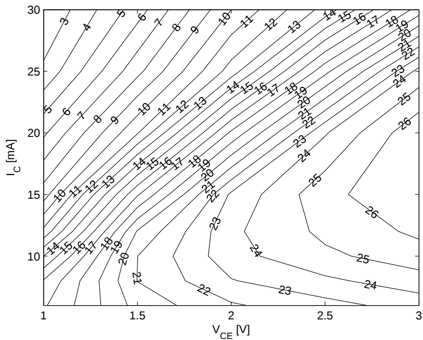
Figure 5-9 3rd Order Intercept Point at output OIP3 [dBm] = f(I_C, V_{CE}) , Z_S = Z_L = 50 \Omega , f = 3.5 \text{ GHz}
