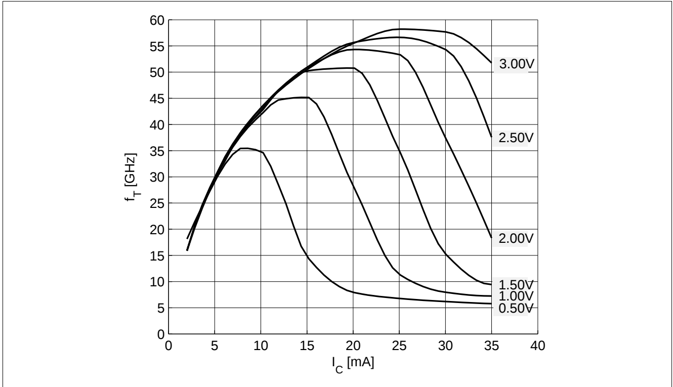
Figure 5-7 Transition Frequency f_T = f(I_C) , f = 1 GHz, V_{CE} = \text{Parameter}
