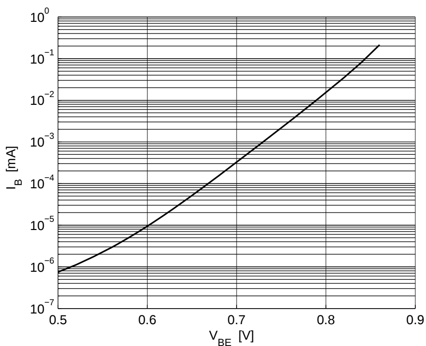
Figure 5-5 Base Current vs. Base Emitter Forward Voltage I_B = f(V_{BE}) , V_{CE} = 2.5 V
