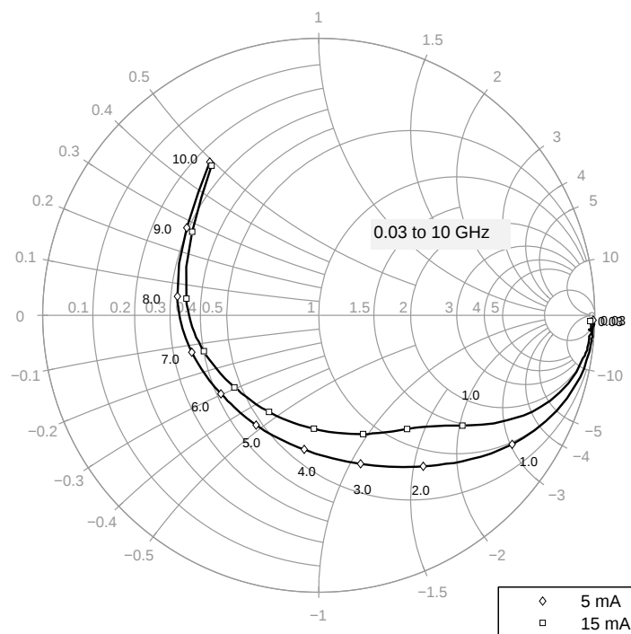
Figure 5-18 Output Reflection Coefficient S_{22} = f(f) , V_{CE} = 2.5\text{ V} , I_C = 5 / 15\text{ mA}
