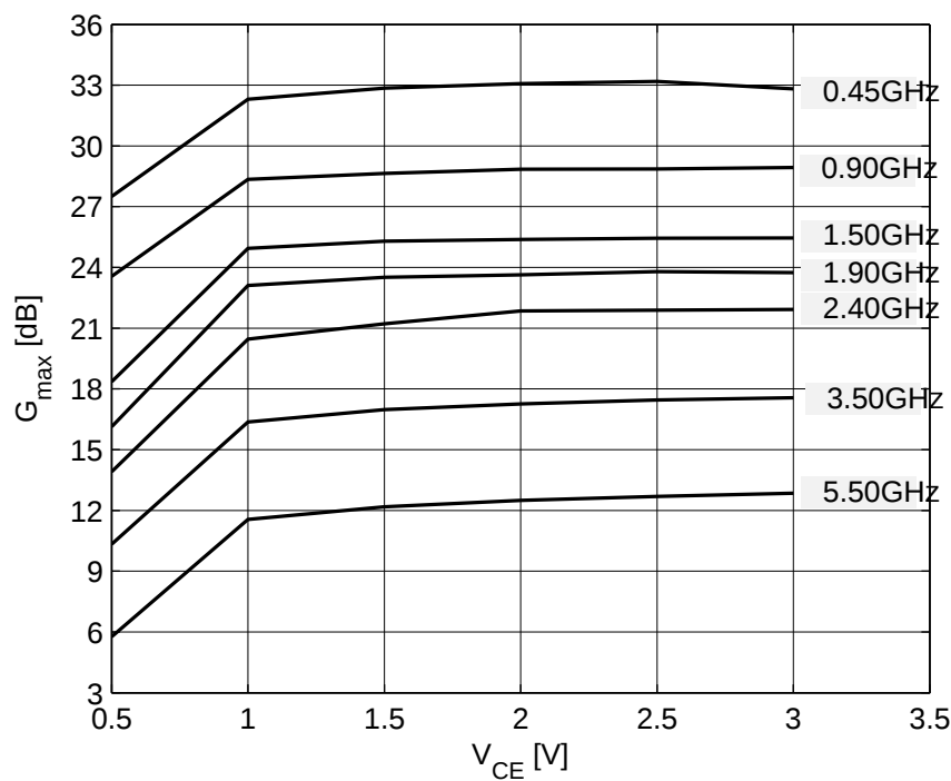
Figure 5-14 Maximum Power Gain G_{\max} = f(V_{CE}) , I_C = 15\text{ mA} , f = \text{Parameter in GHz}
