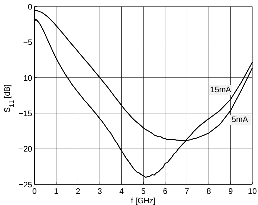
Figure 5-17 Input Reflection Coefficient S_{11} = f(f) , V_{CE} = 2.5\text{ V} , I_C = 5 / 15\text{ mA}
