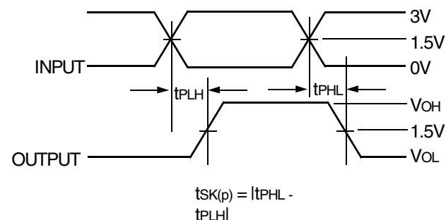
Pulse Skew - t_{SK(P)}
