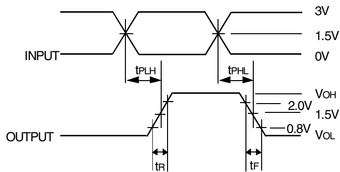
Package Delay
