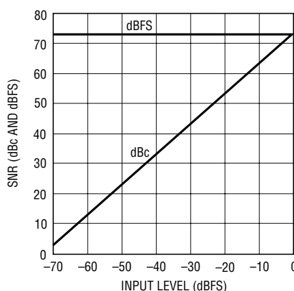
SNR vs Input Level, f_{IN} = 70\text{MHz} , 2V Range, 80Msps
