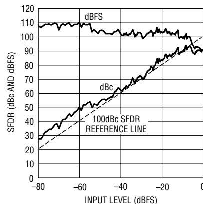
SFDR vs Input Level, f_{IN} = 70\text{MHz} , 2V Range, 80Msps
