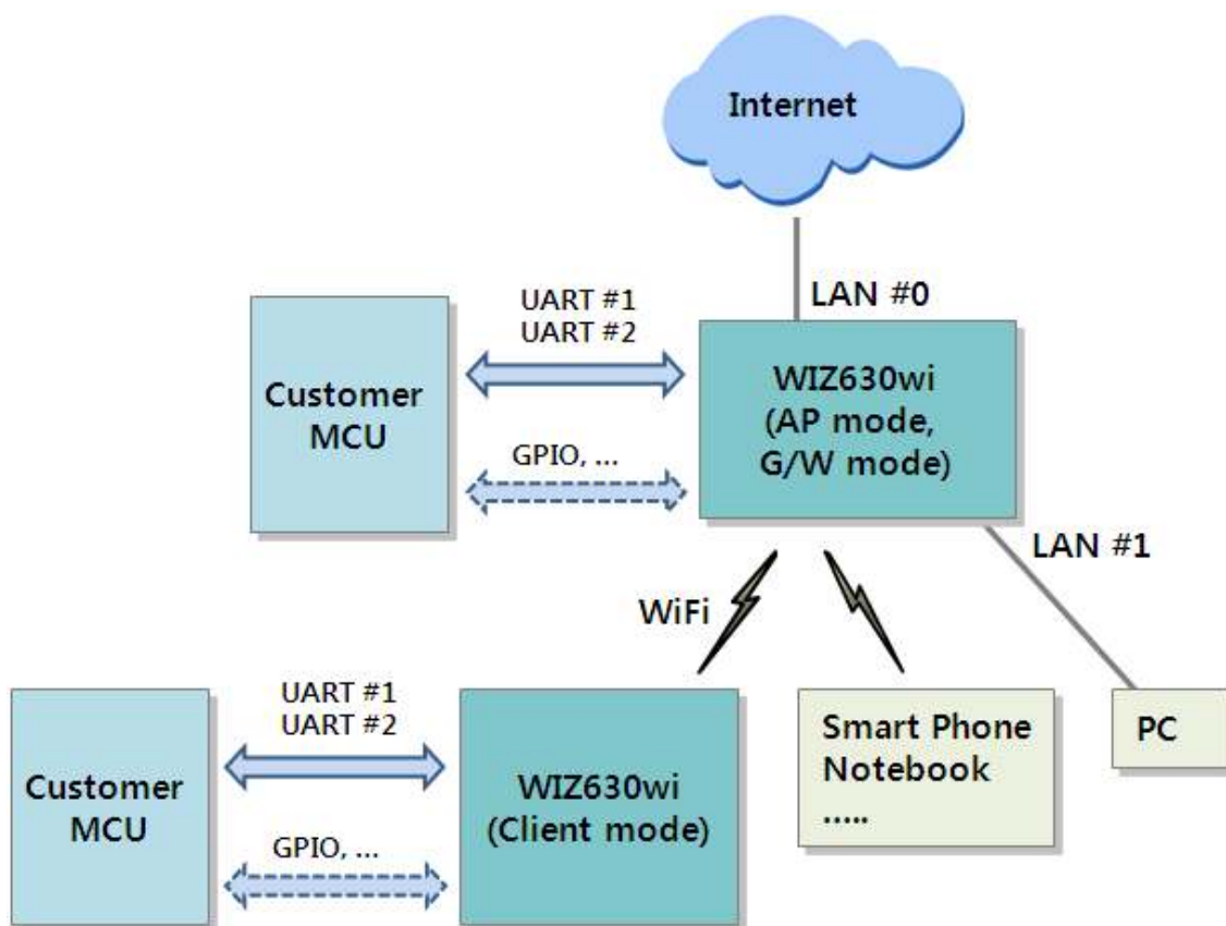
Figure 3. WIZ630wi Functions
