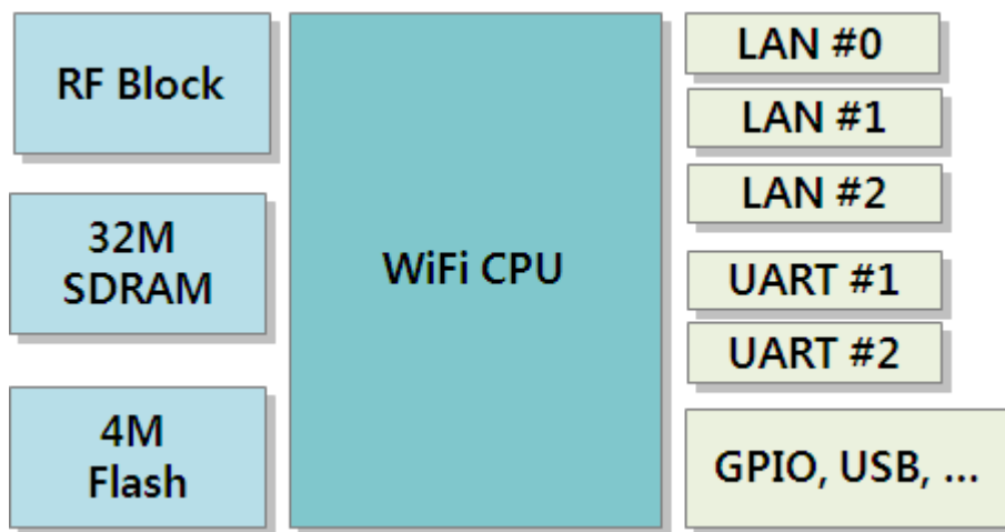
Figure 2. WIZ630wi Interface
