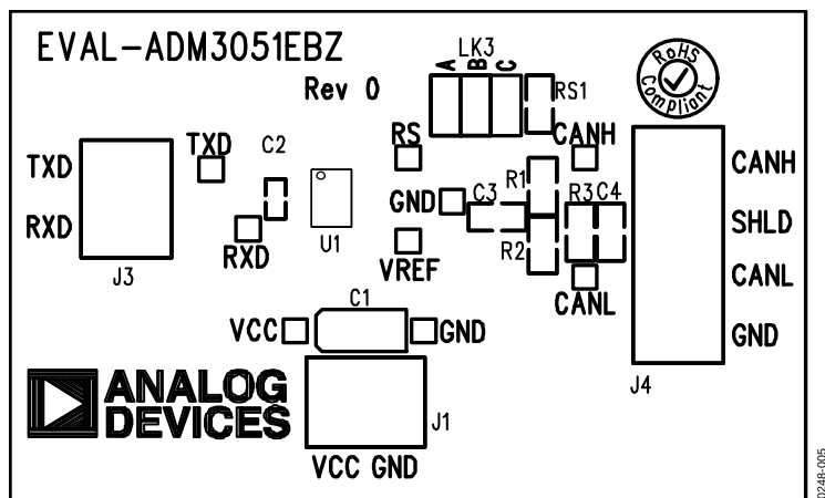
Figure 5. EVAL-ADM3051EBZ Silkscreen
