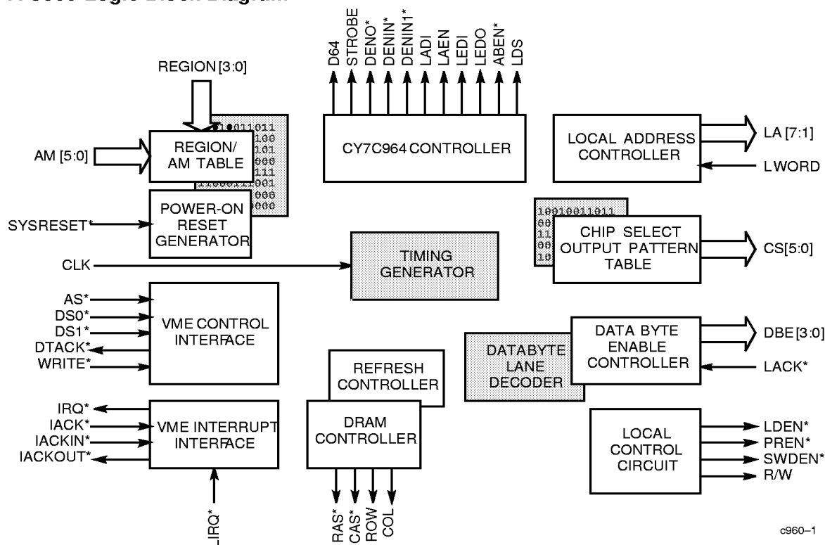
CY7C960 Logic Block Diagram
