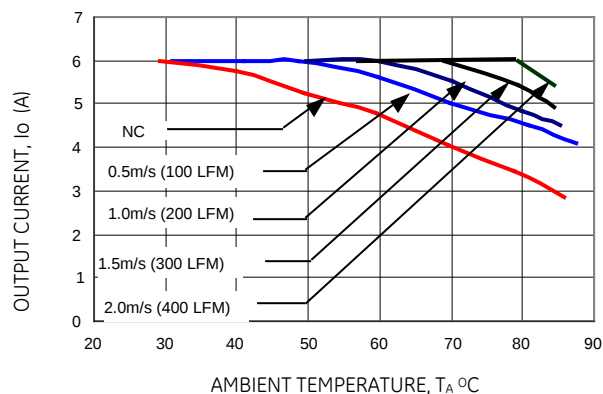
Figure 20. Derating Output Current versus Local Ambient Temperature and Airflow ( V_{in} = 12Vdc , V_o=1.8 Vdc ).
