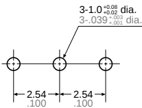
PC board pattern
