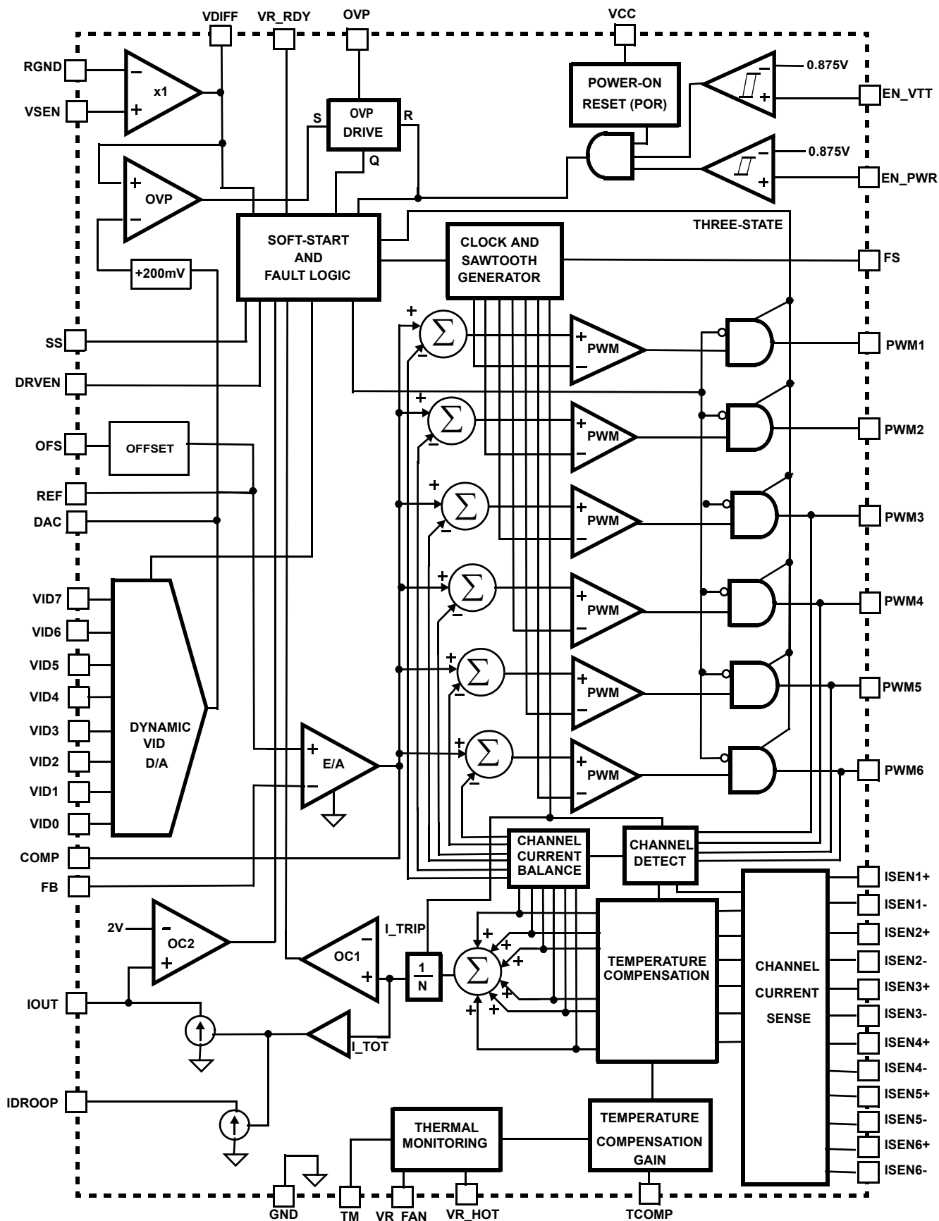
ISL6307A Block Diagram
