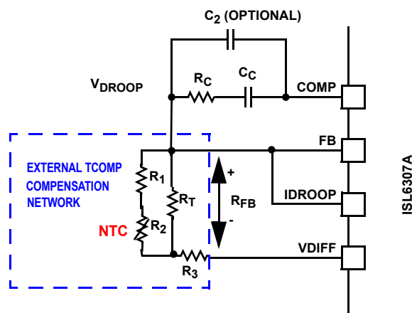
FIGURE 22. TEMPERATURE COMPENSATION WITH EXTERNAL NTC NETWORK
