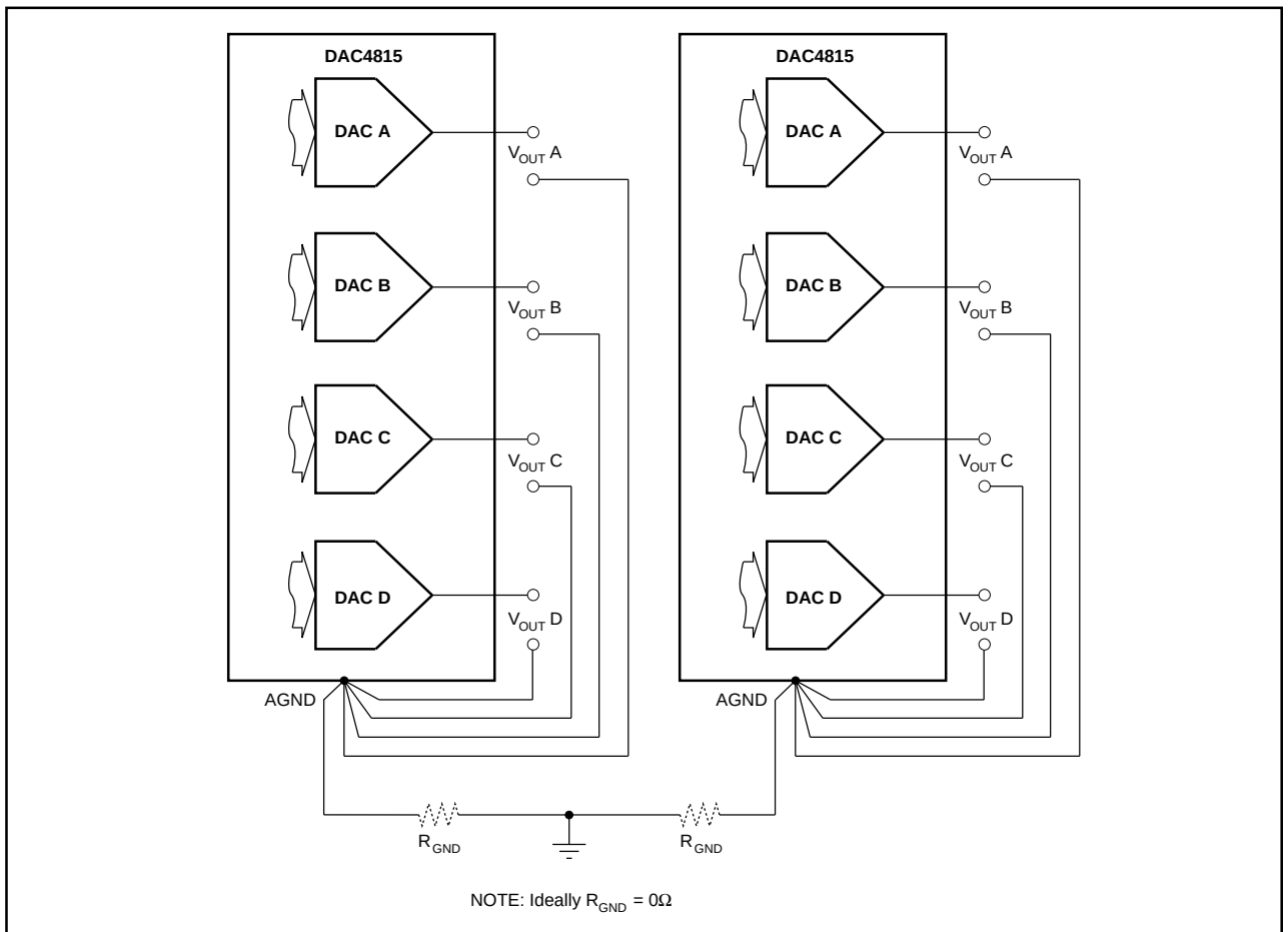
FIGURE 2. Recommended Ground Connections for Multiple DAC Packages.
