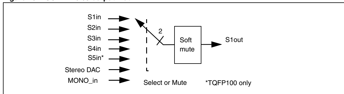
Figure 18. SCART 1/2/3 output matrix
