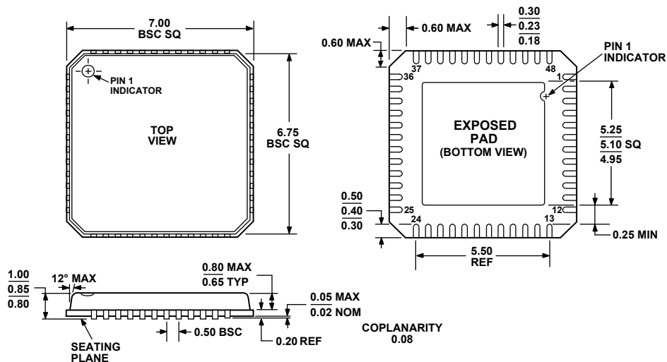
COMPLIANT TO JEDEC STANDARDS MO-220-VKGD-2 Figure 56. 48-Lead Lead Frame Chip Scale Package [LFCSP_VQ] 7 mm × 7 mm Body, Very Thin Quad (CP-48-1) Dimensions shown in millimeters
