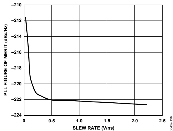
Figure 10. PLL Figure of Merit (FOM) vs. Slew Rate at \overline{\text{REFIN}}/\text{REFIN}
