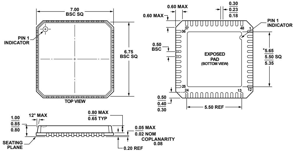
*COMPLIANT TO JEDEC STANDARDS MO-220-VKGD-2 WITH EXCEPTION TO EXPOSED PAD DIMENSION. Figure 55. 48-Lead Lead Frame Chip Scale Package [LFCSP_VQ] 7 mm × 7 mm Body, Very Thin Quad (CP-48-8) Dimensions shown in millimeters
