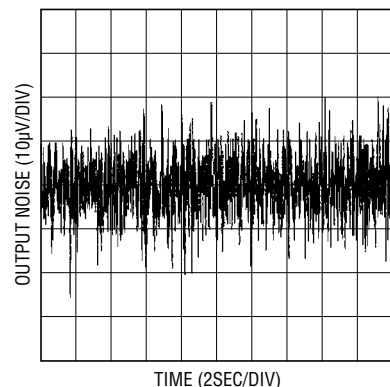
5V Output Noise 0.1Hz ≤ f ≤ 10Hz
