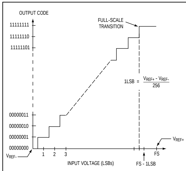
Figure 10. Transfer Function
