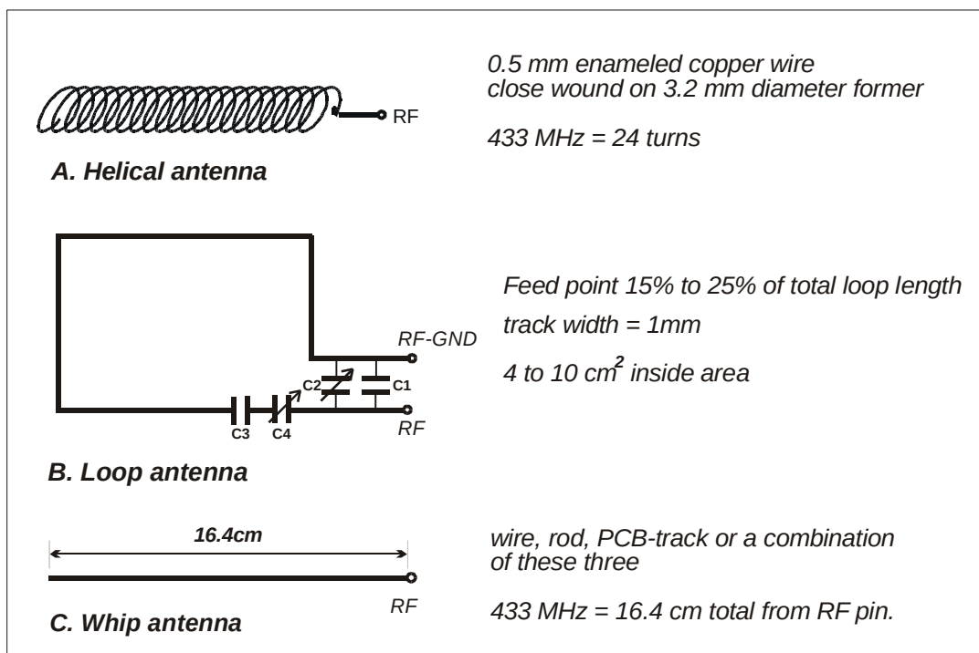
Fia.8: Antenna
